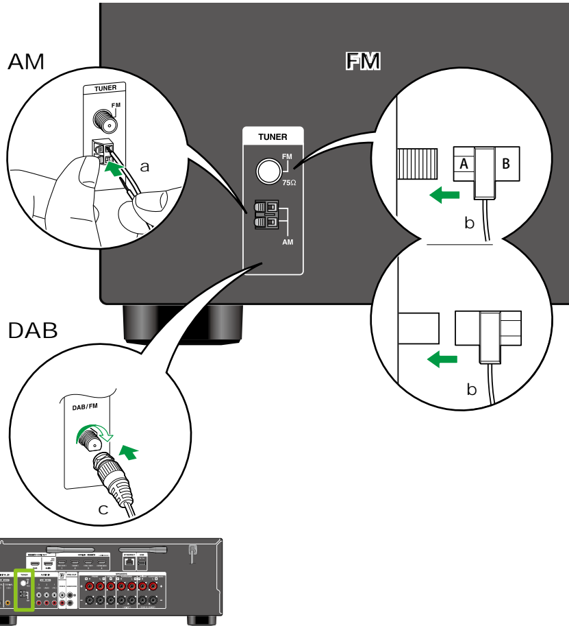
a AM loop antenna, b Indoor FM antenna, c DAB/FM antenna
