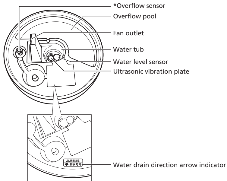
Water tank back side
